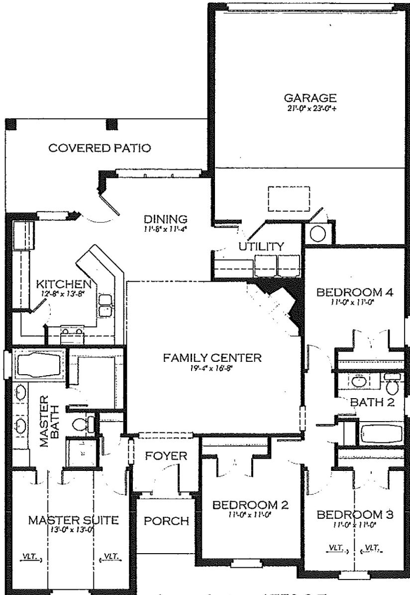
LIVING AREA — 1759 S.F.
