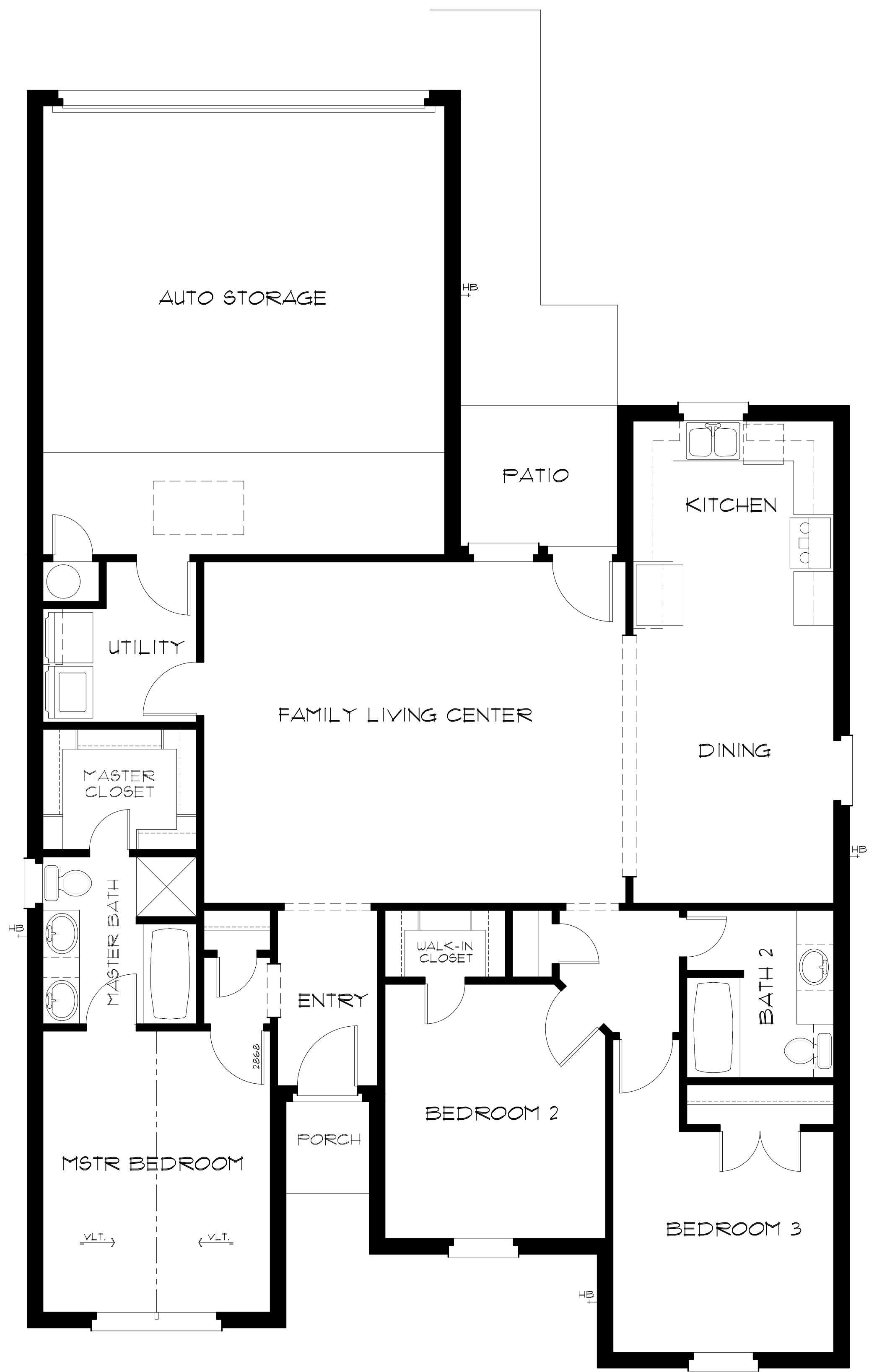
FLOOR PLAN
